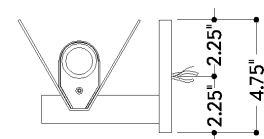
SIDE
