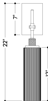
FRONT
