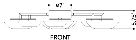
FRONT
