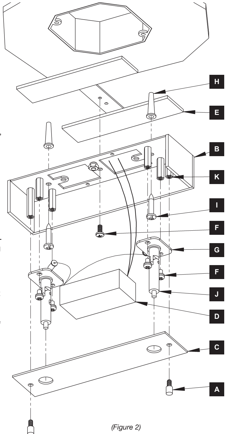
(Figure 2) Canopy side plate hidden to show inside of canopy.
