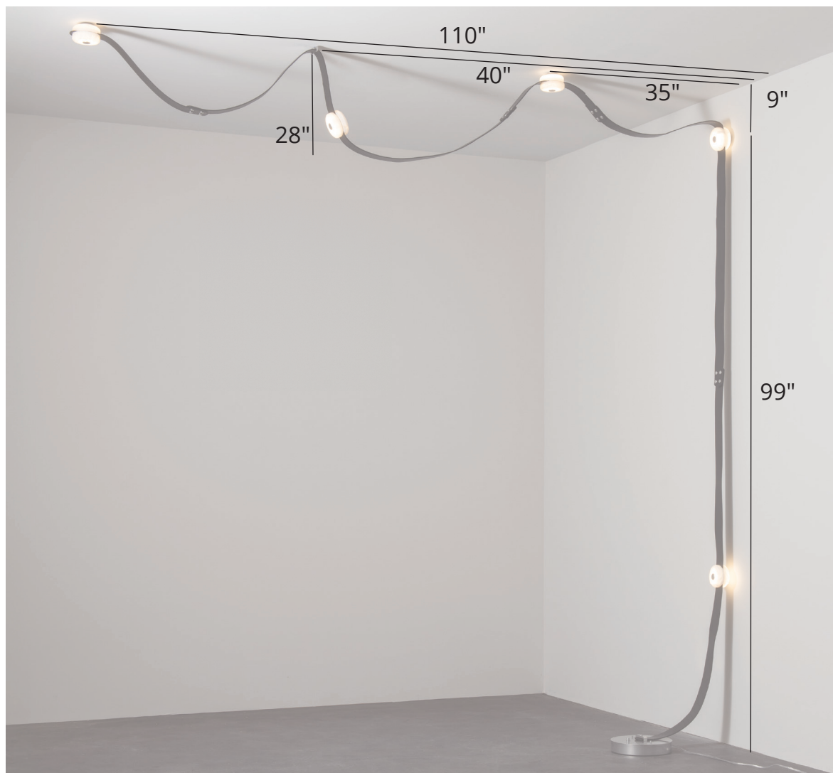
SNAPS PLUG-IN LED LAMP · 402801 WITH 24" STRAP AND LED 905701 & 72" STRAP AND LED 905713 Configuration 4 · 108" h x 36" w x 10.5" d
