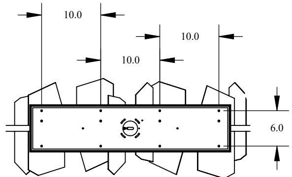
MOUNTINGDETAIL SCALE 1 : 16
