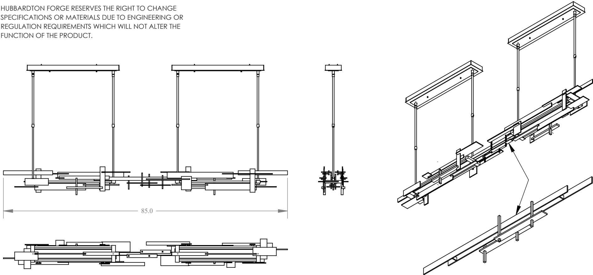
LOOSE CONNECTOR ASSEMBLY SITS ON TOP OF TWO SEPARATE FIXTURES
