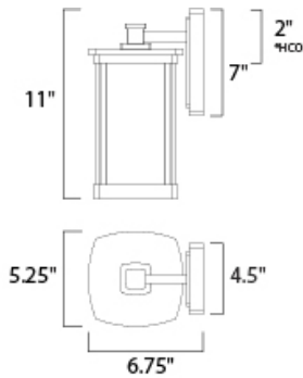
*height from center of outlet to top of the fixture
