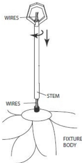
DRAWING 3-Stem install
