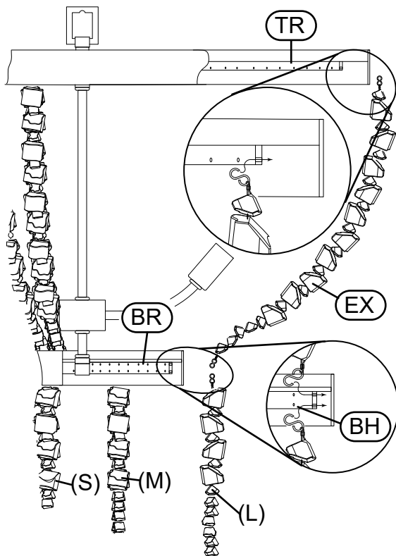
DRAWING 2 - GLASS INSTALLATION
