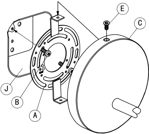
DRAWING 1 - MOUNTING
