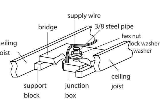
DRAWING 2 - installation example
