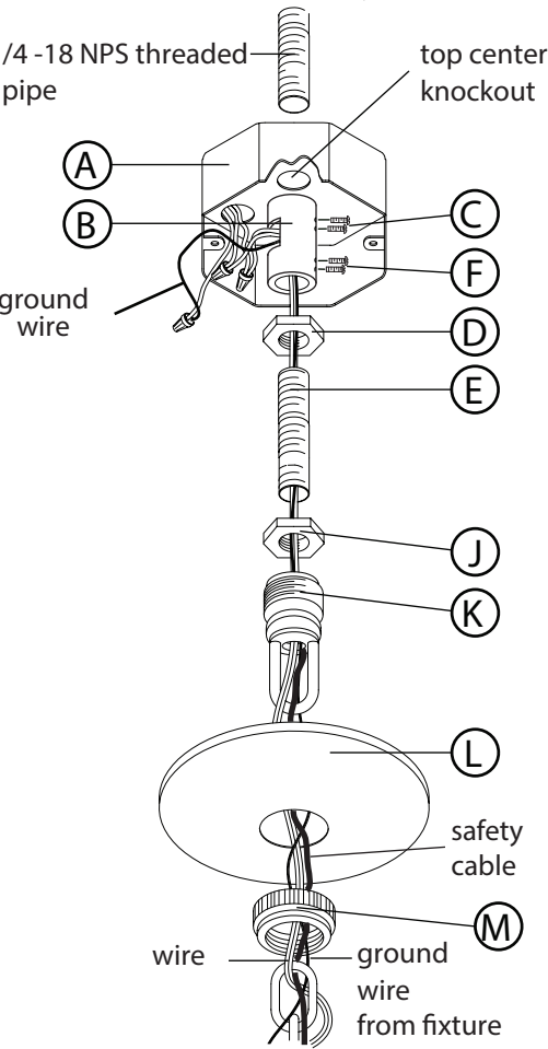
DRAWING 1 - MOUNTING
