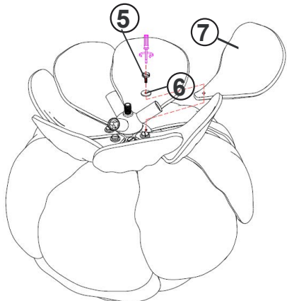
Drawing 3- Pedal Assembly
