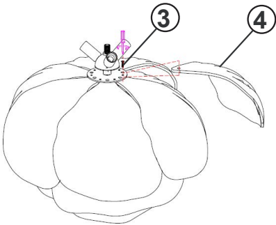
Drawing 3- Pedal Assembly
