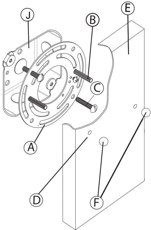
DRAWING 2- SHADE INSTALLATION
