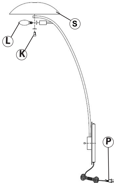
DRAWING 2- SHADE INSTALLATION
