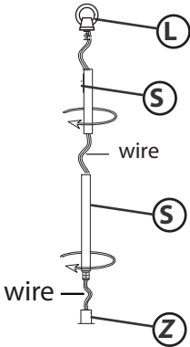
Drawing 1 – Stem Assembly
