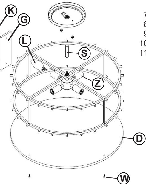
DRAWING 2 - Assembly
