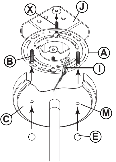
DRAWING 2 - Assembly
