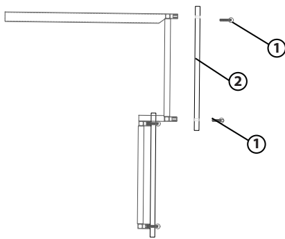
Drawing 2- Panel install
