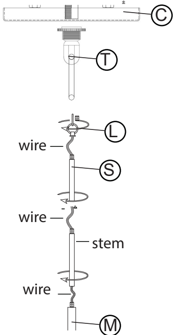
Drawing 2- Panel install
