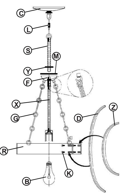
Drawing 1 – Assembly
