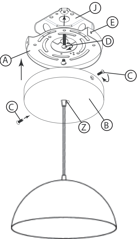
DRAWING 1 - MOUNTING
