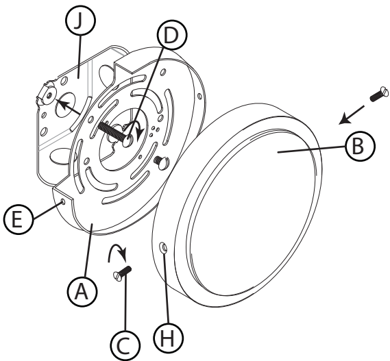
DRAWING 1 - MOUNTING
