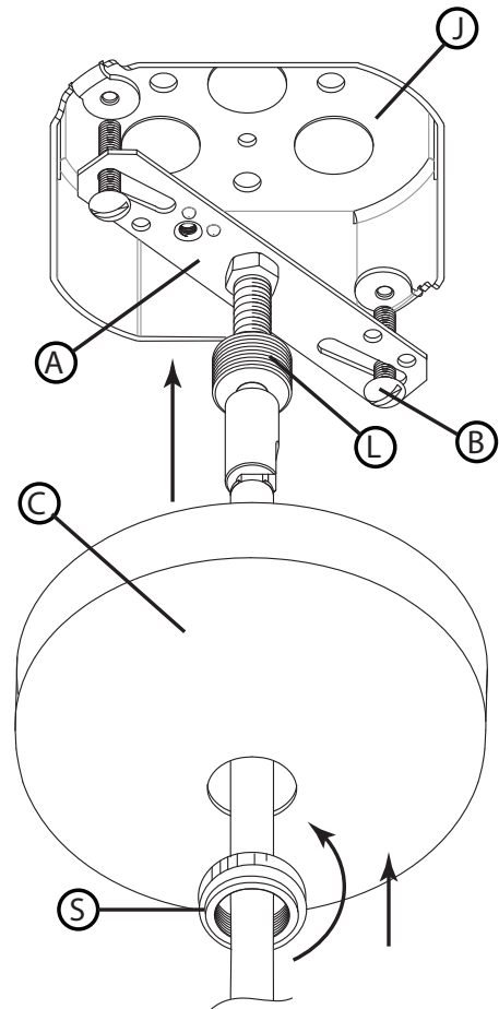
Drawing 1 - Fixture Mounting
