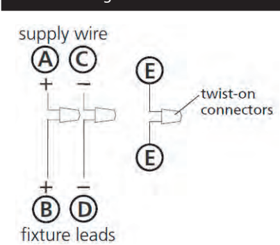
Drawing 3 – Post-Mount
