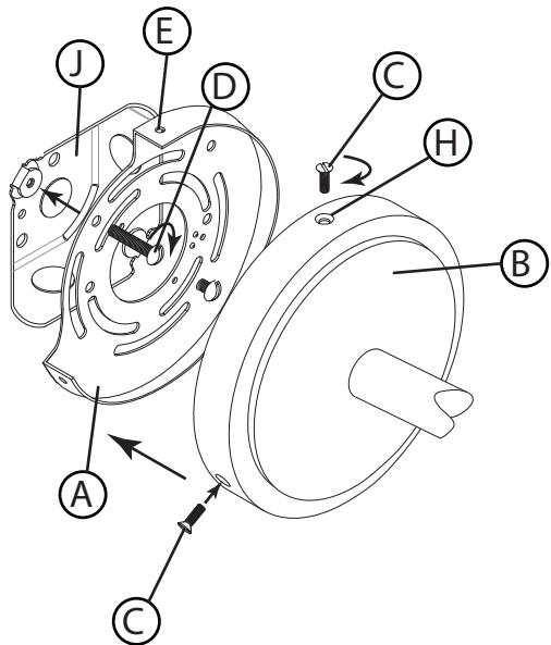
DRAWING 1 - MOUNTING
