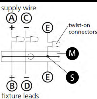
Drawing 3 – Post-Mount
