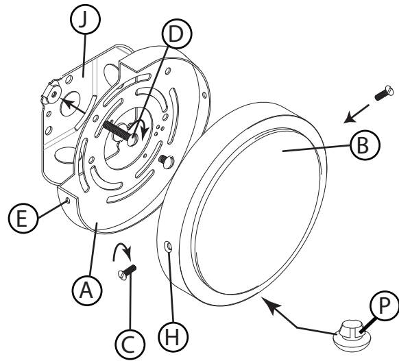
Drawing 2- Fixture diagram
