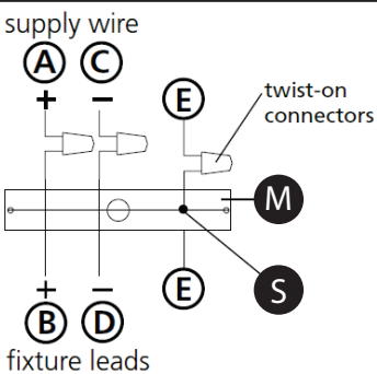
Drawing 3 – Post-Mount
