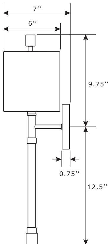
SIDE VIEW
