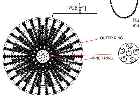
BOTTOM VIEW OF BOTTOM RING
