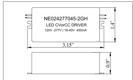
LED DRIVER DIAGRAM
