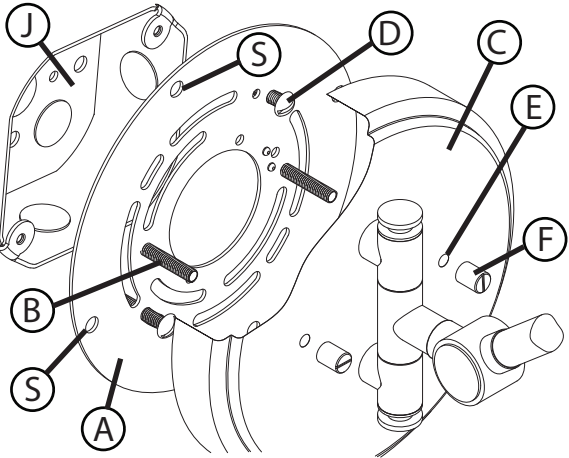
DRAWING 2 - FIXTURE PREPERATION
