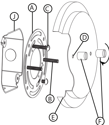
DRAWING 1 - MOUNTING
