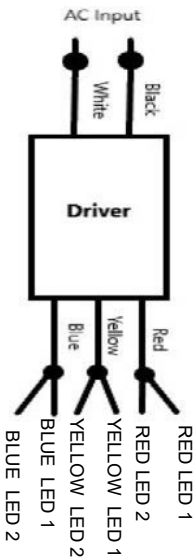
Drawing 4- Electrical connections 2 drivers
