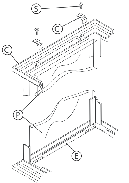
DRAWING 2 - MOUNTING
