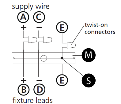
Drawing 3 – Post-Mount
