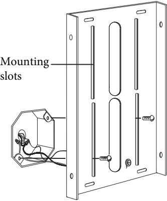
SG-ADAPT1-Single Gang Box Adaptor Plate
