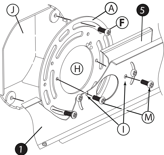
DRAWING 3 - MOUNTING
