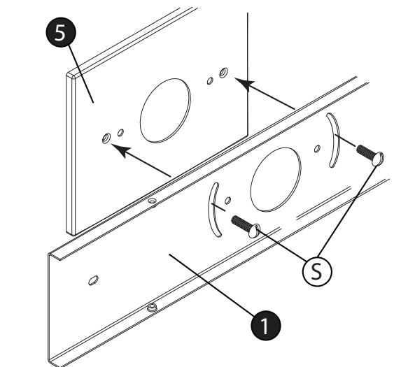
DRAWING 3 - MOUNTING
