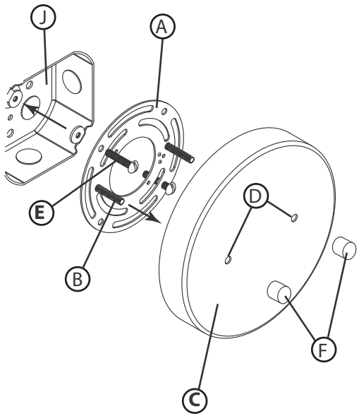
DRAWING 2 - FIXTURE PREPERATION
