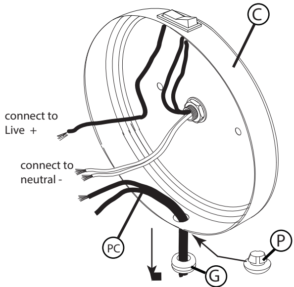
DRAWING 2 - FIXTURE PREPERATION
