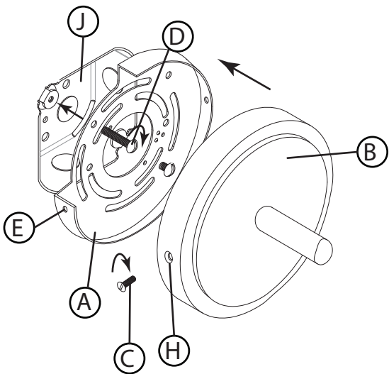
DRAWING 1 - MOUNTING
