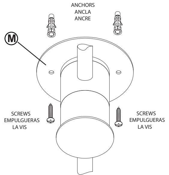
DRAWING 1 - MOUNTING P2 POINT
