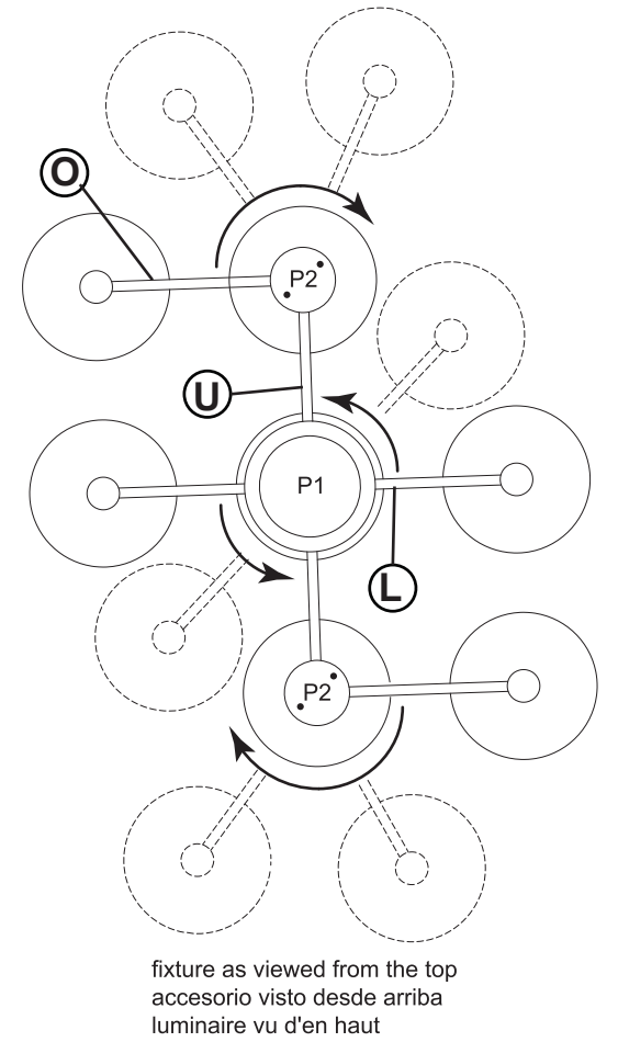
DRAWING 1 - MOUNTING P2 POINT
