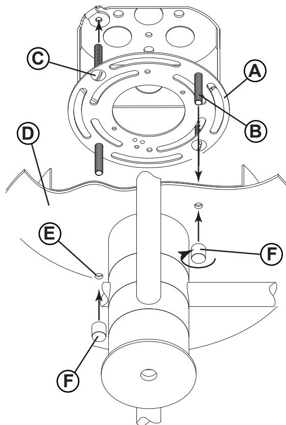
DRAWING 2 - MOUNTING
