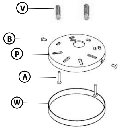
Drawing 2 - Mounting with junction box
