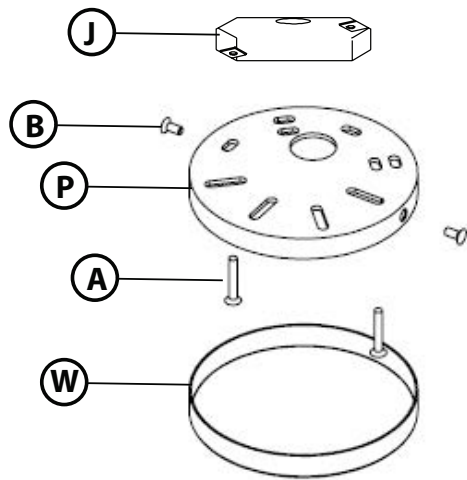
Drawing 3-Glass Install
