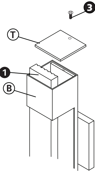
DRAWING 2 - ASSEMBLY
