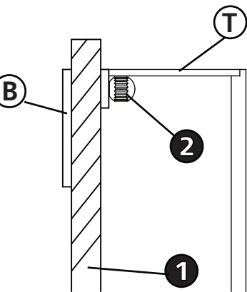
DRAWING 2 - ASSEMBLY
