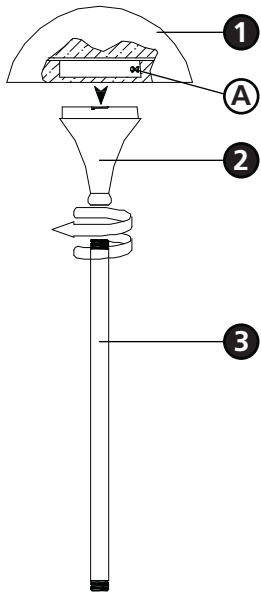
Drawing 1 - Fixture Mounting
