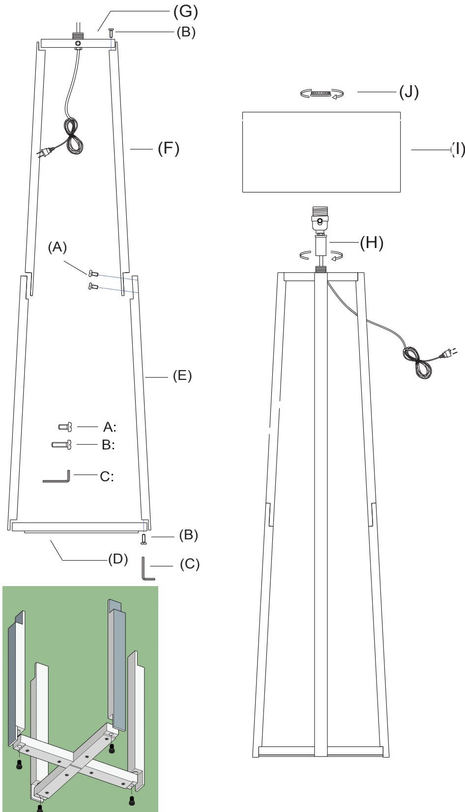
FIG 1: BASE ASSEMBLY Bottom of base facing floor
