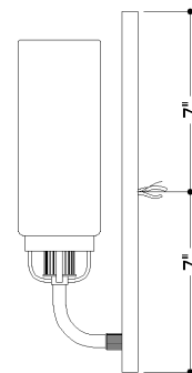
SIDE
