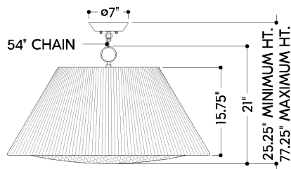
FRONT
